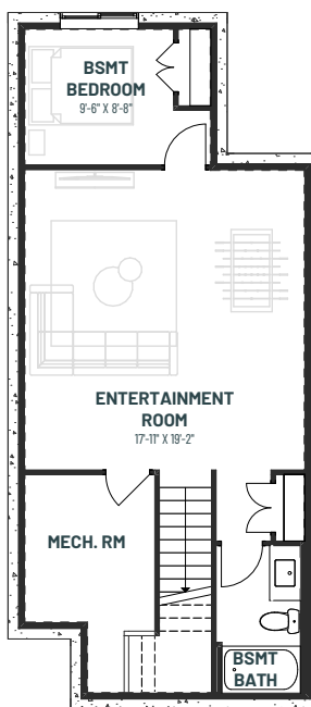
BASEMENT DEVELOPMENT OPTION 574 SQ. FT.
