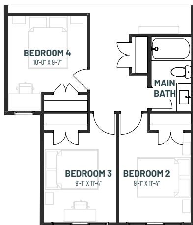
SECOND FLOOR OPTION 4th Bedroom
