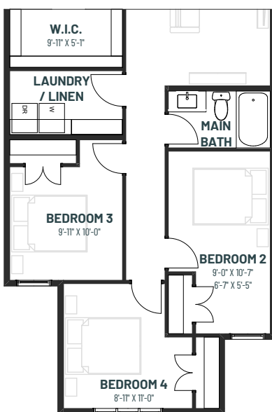
SECOND FLOOR OPTION 4th Bedroom 1,340 SQ.FT.
