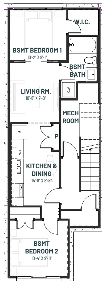
SECONDARY SUITE OPTION 674 SQ.FT.
