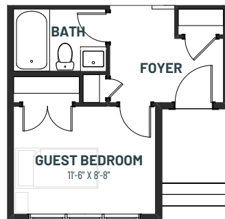
MAIN FLOOR OPTION Guest Bed & Bath
