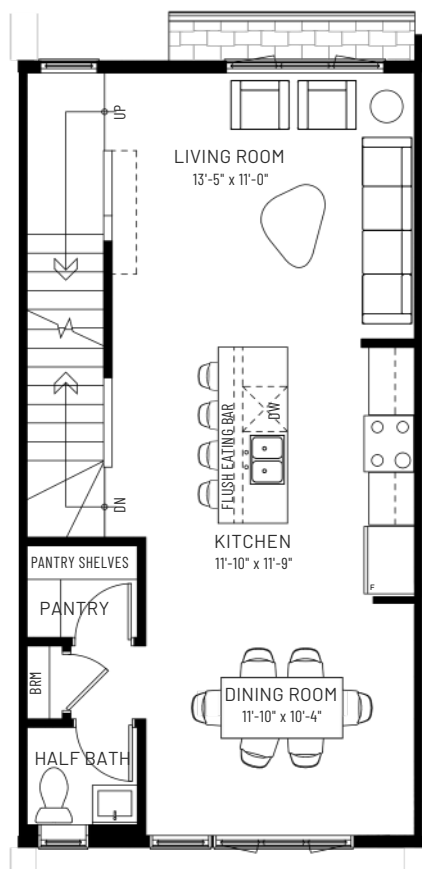
MAIN FLOOR CENTER KITCHEN 630 SQ.FT.
