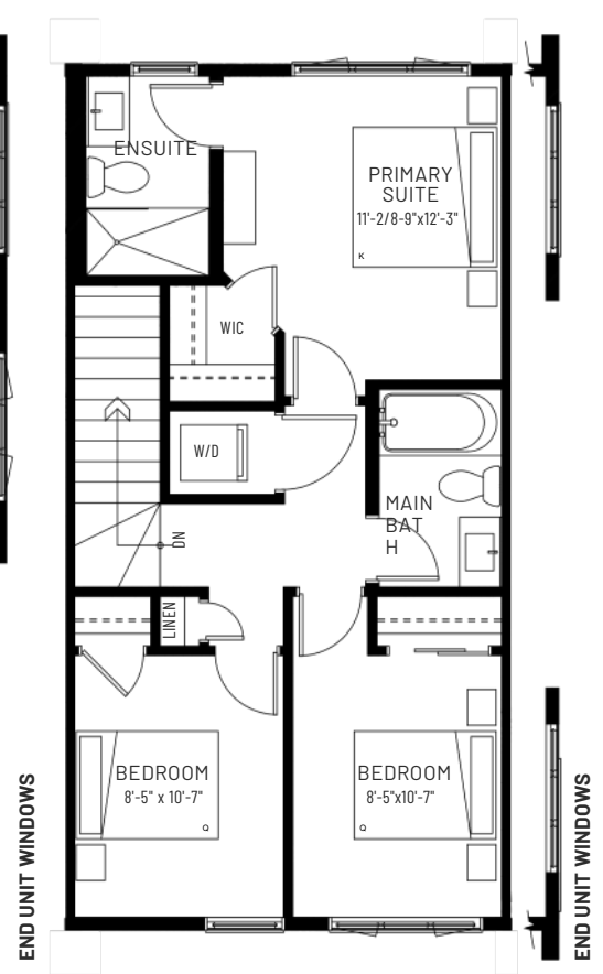
UPPER FLOOR 587 SQ.FT.
