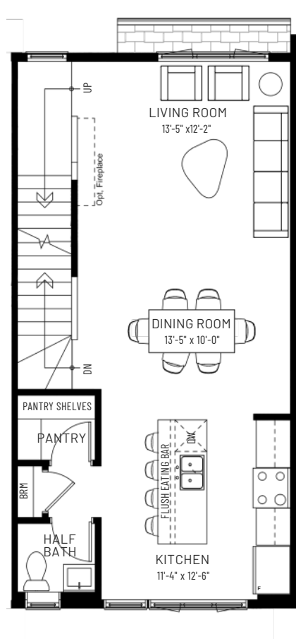
MAIN FLOOR 630 SQ.FT.
