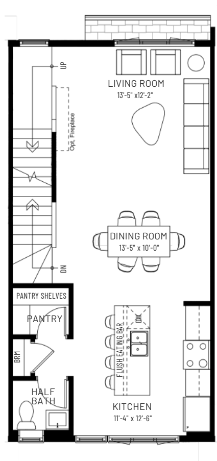
MAIN FLOOR 692 SQ.FT.
