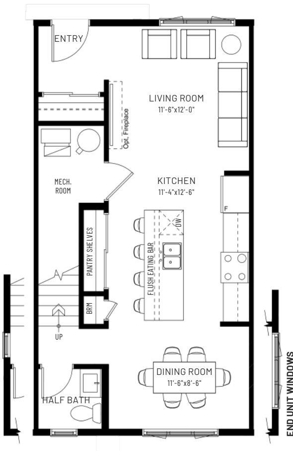
MAIN FLOOR 623 SQ.FT.
