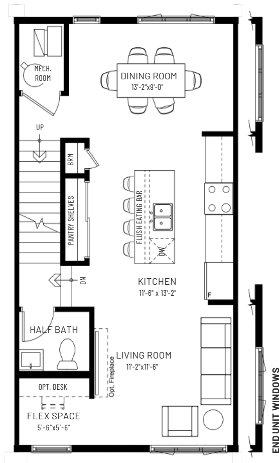
MAIN FLOOR 630 SQ.FT.
