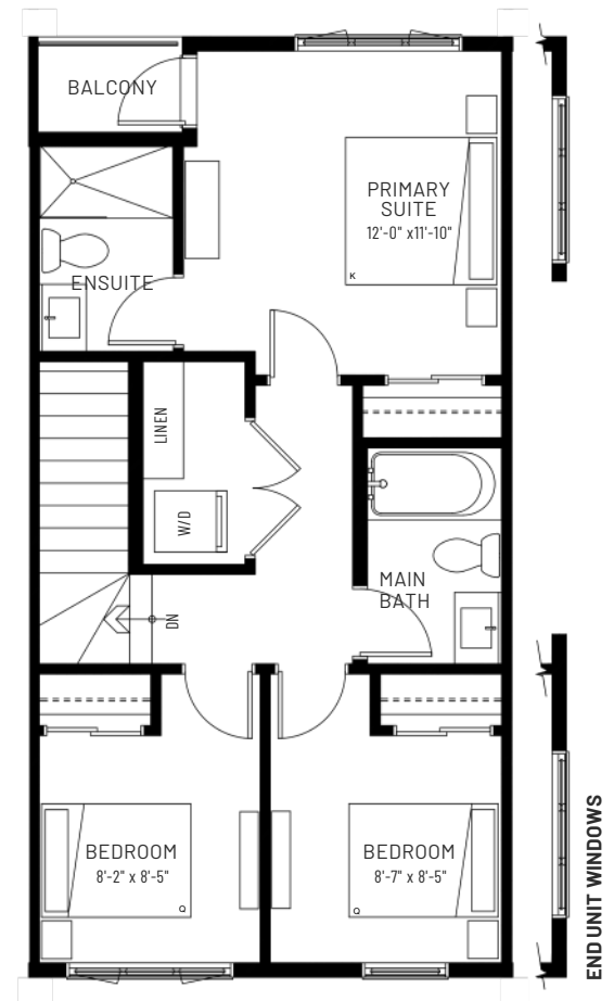
UPPER FLOOR 564 SQ.FT.
