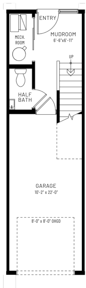
GROUND FLOOR 126 SQ.FT.
