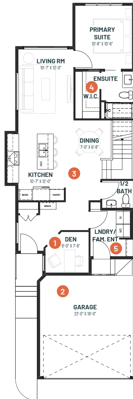
MAIN FLOOR 992 SQ.FT.
