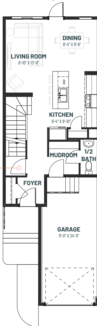
MAIN FLOOR 584 SQ.FT.
