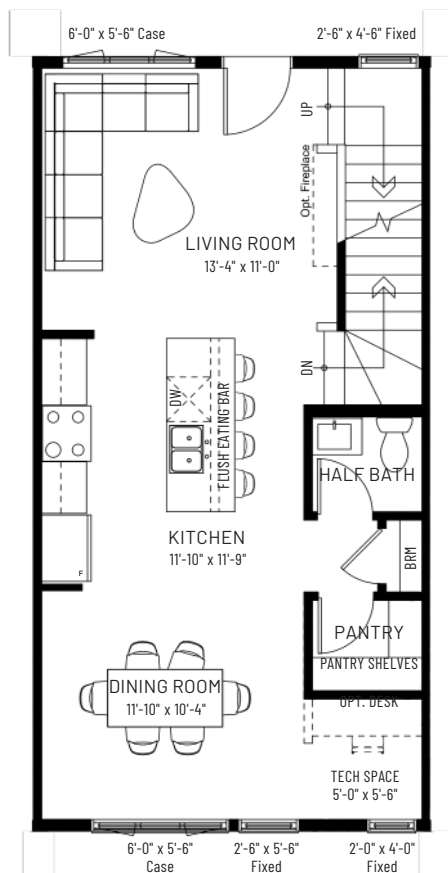
MAIN FLOOR CENTER KITCHEN 630 SQ.FT.
