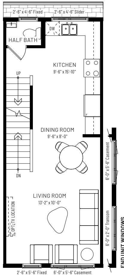
MAIN FLOOR 490 SQ.FT.
