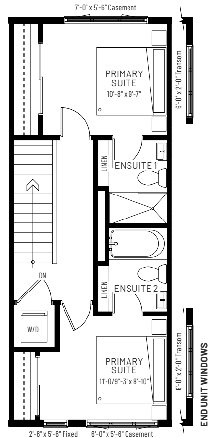
UPPER FLOOR OPTION 450 SQ.FT.
