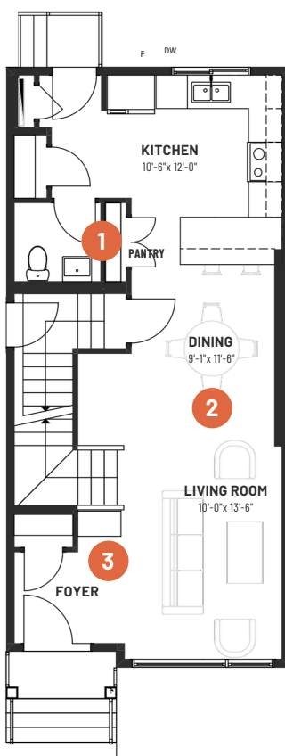
MAIN FLOOR 677 SQ.FT.
