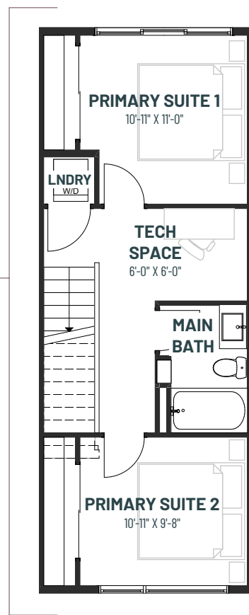
UPPER FLOOR- TECH SPACE OPTION
