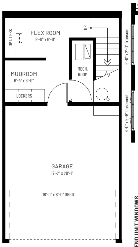
GROUND FLOOR 174 SQ.FT.
