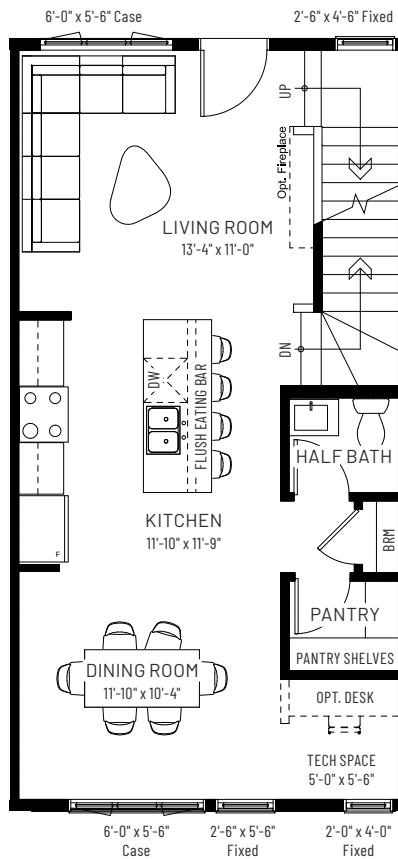
MAIN FLOOR CENTER KITCHEN 630 SQ.FT.
