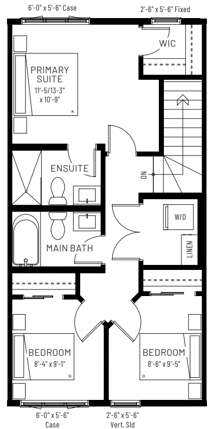
UPPER FLOOR 587 SQ.FT.
