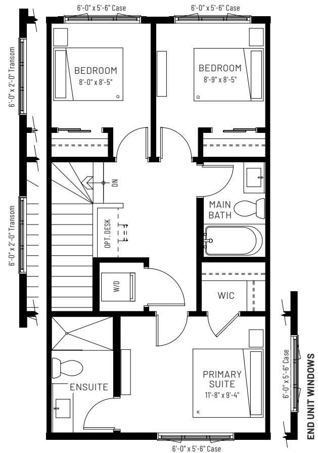
UPPER FLOOR 579 SQ.FT.
