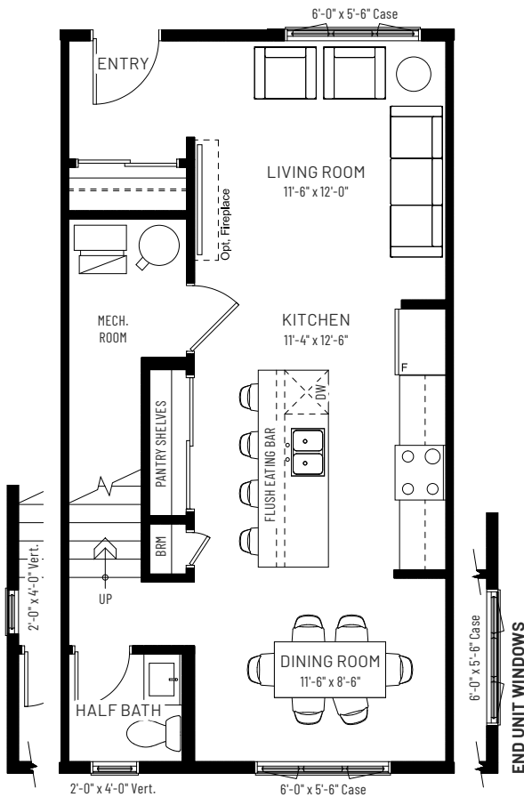
MAIN FLOOR 623 SQ.FT.
