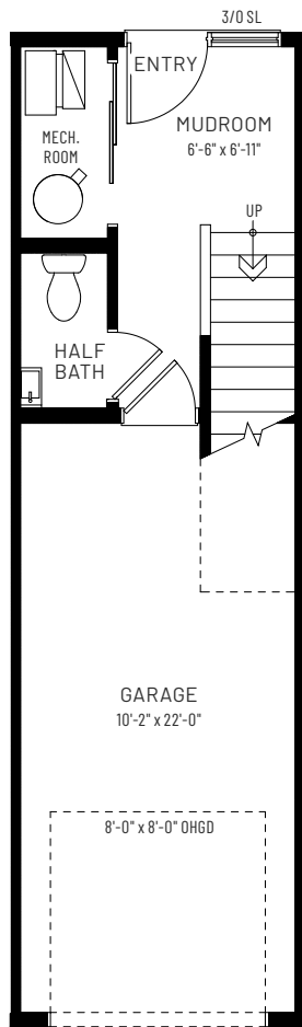
GROUND FLOOR 126 SQ.FT.
