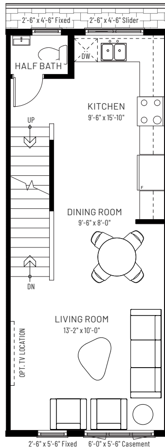
MAIN FLOOR 490 SQ.FT.
