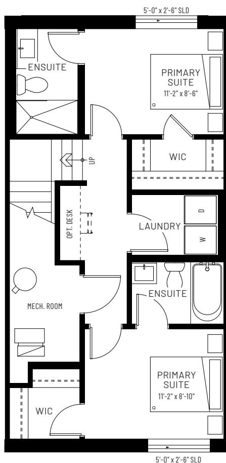
BASEMENT 487 SQ.FT.
