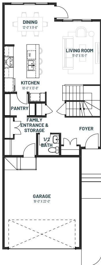
EXTENDED LIVING ROOM OPTION 834 SQ.FT.
