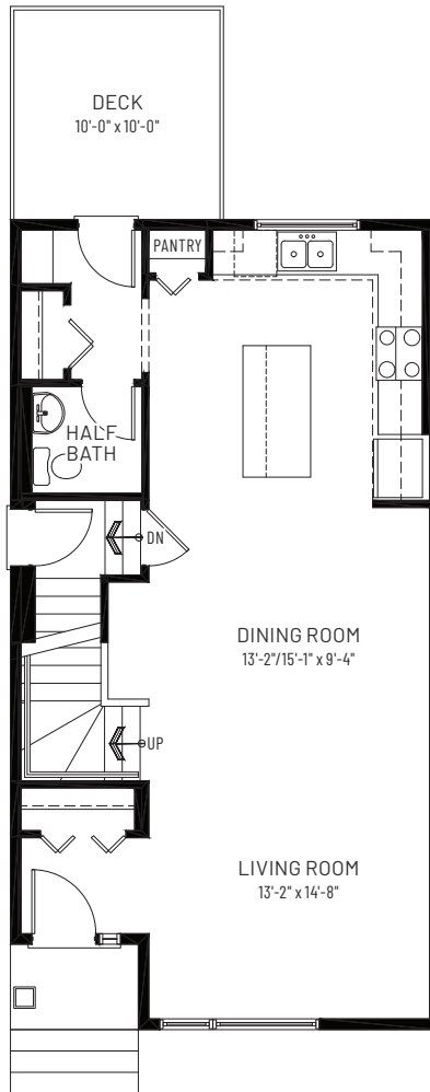
MAIN FLOOR (OPTION) 738 SQ.FT.
