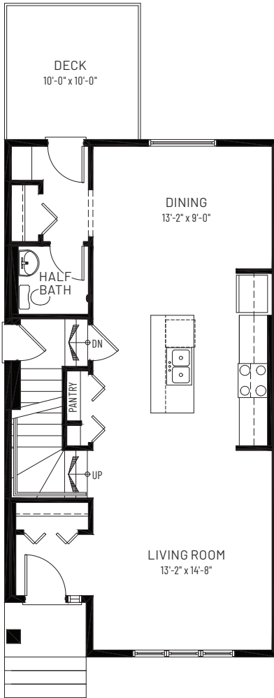
MAIN FLOOR 738 SQ.FT.
