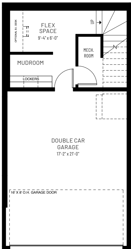
GROUND FLOOR 174 SQ.FT.
