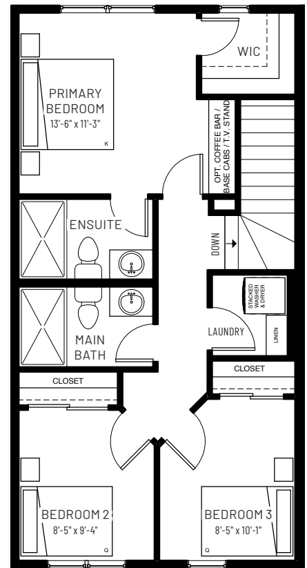
UPPER FLOOR 587 SQ.FT.
