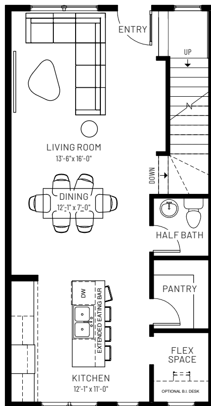
MAIN FLOOR 630 SQ.FT.
