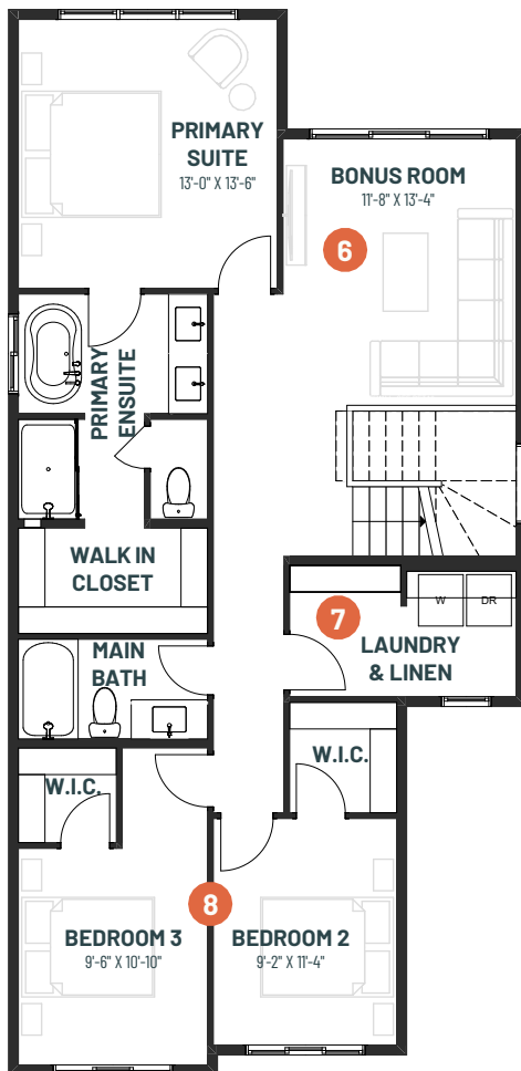
SECOND FLOOR 1,139 SQ.FT.
