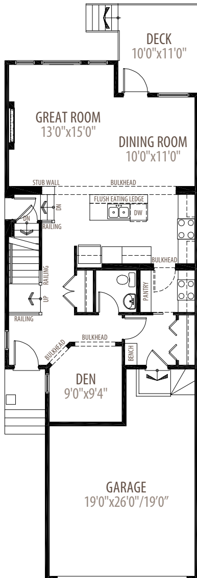
MAIN FLOOR 942 SQ.FT.
