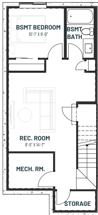
BASEMENT DEVELOPMENT OPTION 503 SQ.FT.
