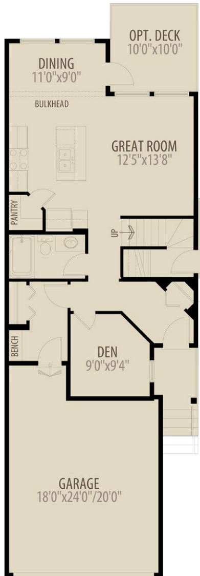
MAIN FLOOR 784 SQ.FT.
