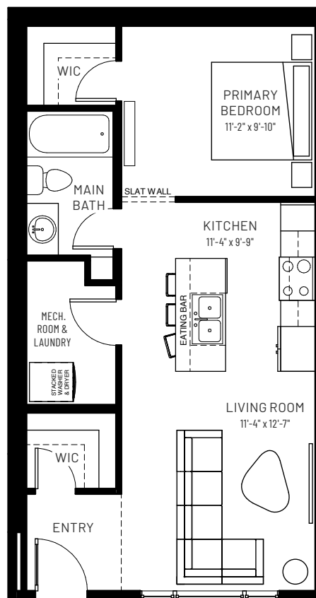
GROUND FLOOR 538 SQ.FT.
