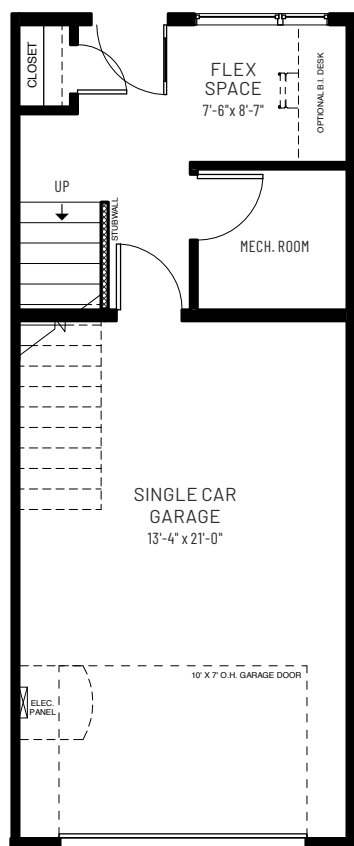
GROUND FLOOR 145 SQ.FT.
