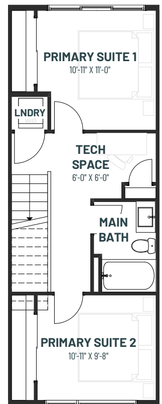
UPPER FLOOR 479 SQ.FT.
