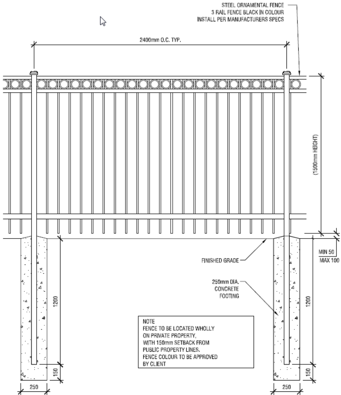
DECORATIVE STEEL FENCE DETAIL N.T.S.
