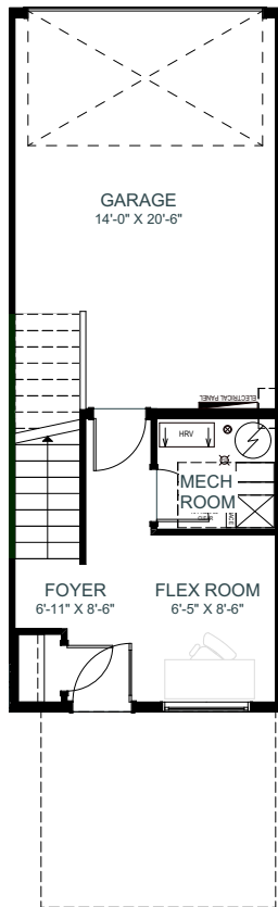
GROUND FLOOR 176 SQ.FT.
