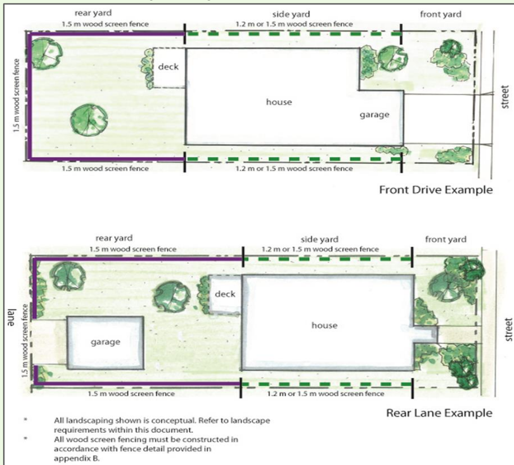
Figure 2: Fencing Plan – Typical Lots
