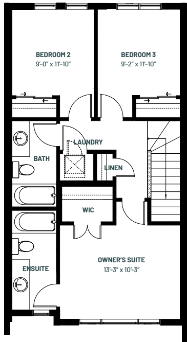
3 BEDROOM + 2.5 BATHS 636 SQ. FT.
