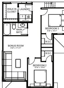
6 Three Bedroom Layout 2
