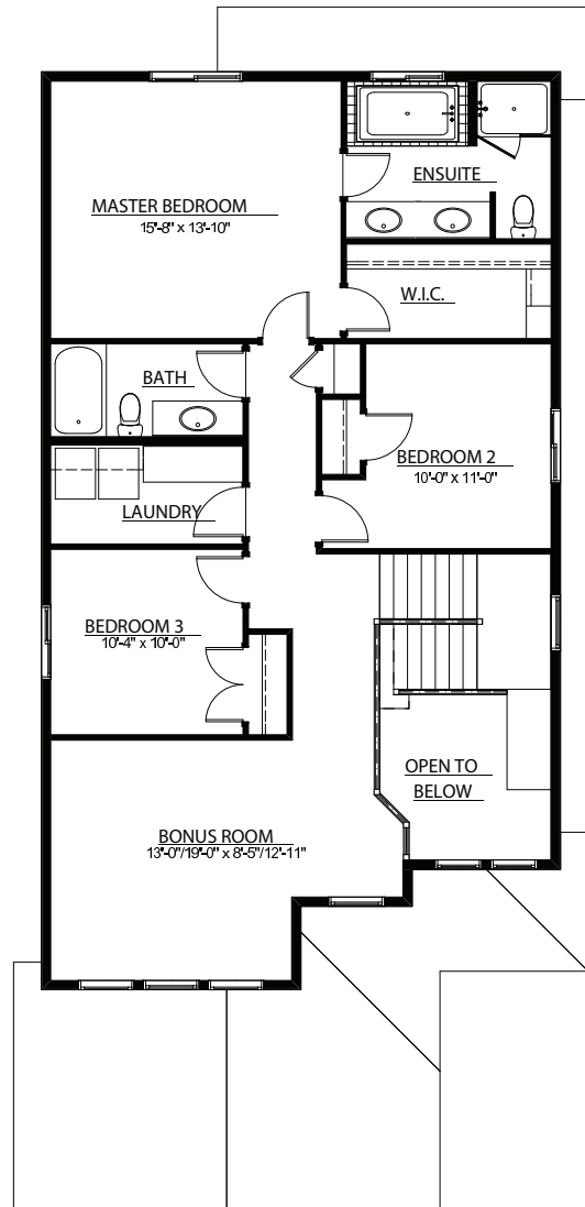
UPPER FLOOR 1196 SQ. FT.
